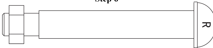
Right M12 x 110mm Allen Bolt (87) & Right M12 Screw Nut (90) Step 6
